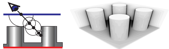
Figure 11: Left: sphere tracing algorithm. Right: example with the number of steps visualized: from white=0 steps to black=40 steps.
