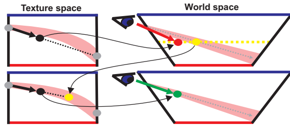
Figure 9: Sampling correction: the sample point is projected into world space and checked for validity (top row). If invalid, we redirect to a closer valid point (bottom row).
