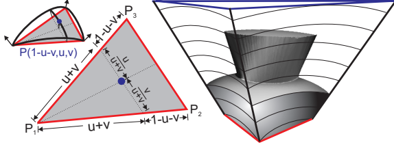
Figure 6: Construction of a curved shell map in world space using Coons patches.
